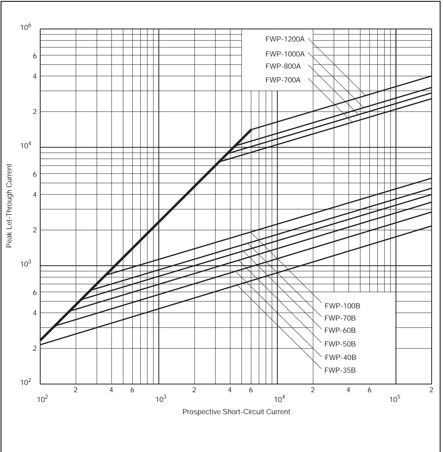
Peak Let-Through Cut-Off Current Characteristic Curves FWP 35B-100B & 700A-1200A
